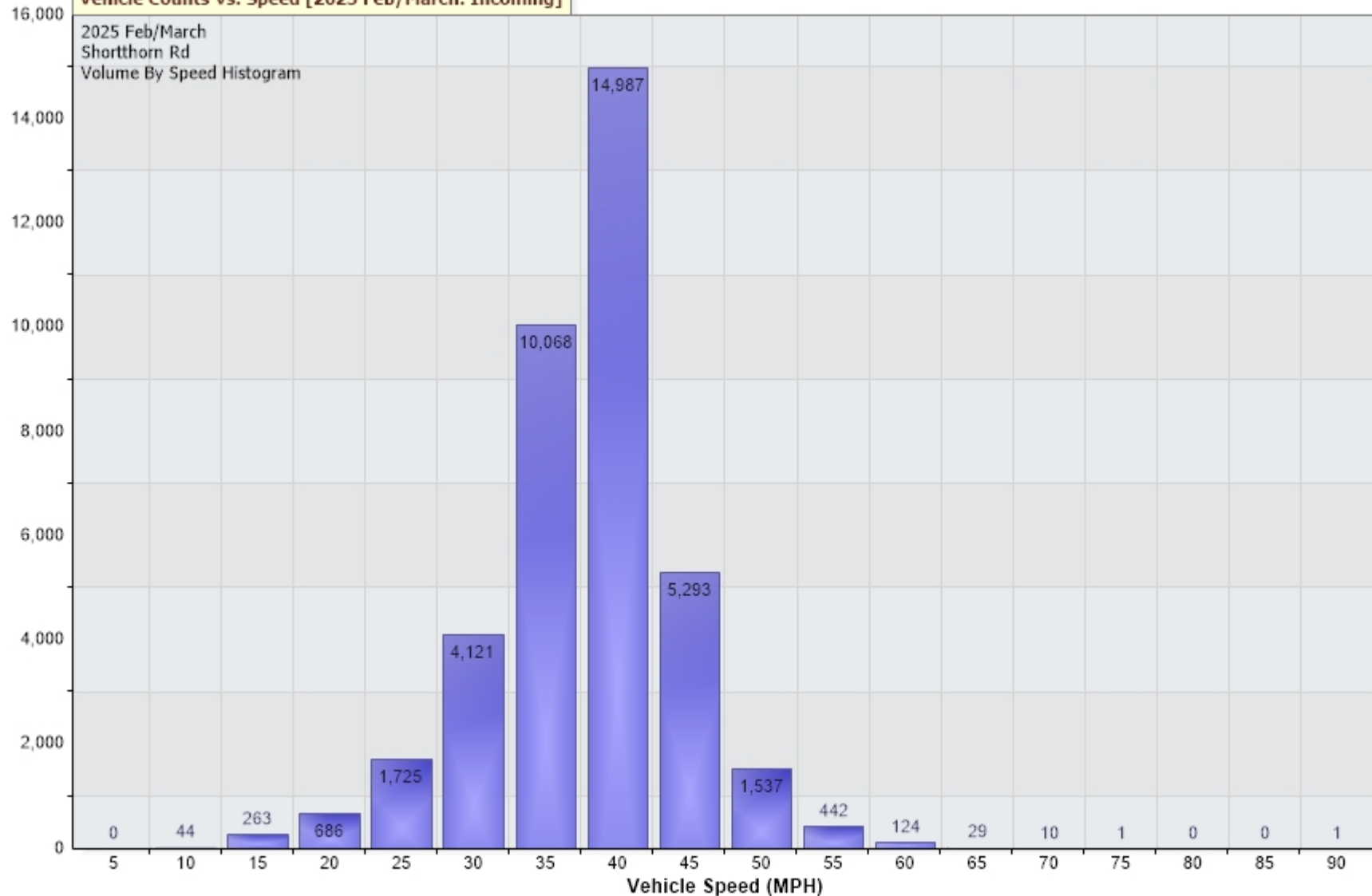
Vehicle Counts Vs. Speed [2025 Feb/March: Incoming]
